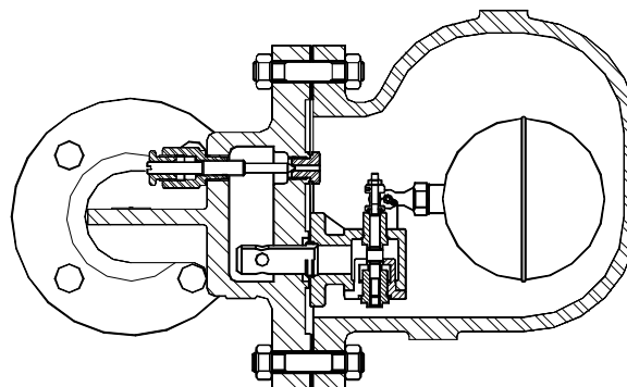
FLT17-FLT32-FLT41 DN25HC
